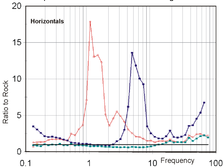
Figure 3A. SSR analysis of the Au Sable Forks spectra at stations OT001, WM, and GH, relative to OTT (black line at value =1), as taken from figure 10 of Al-Khoubbi and Adams (2004).
